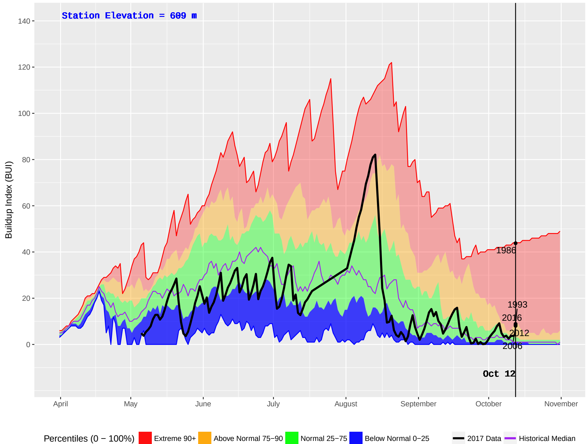
BOB QUINN LAKE (113) : Historical (1984–2016) and Current (2017) Noon Buildup Index (BUI)
